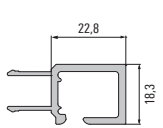
928 129 Linero system rail
