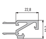
928 130 Lighting profile
