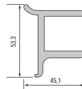
903 011 Base support profile 25 mm
