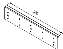
928 069.70.99 Bracket for timber base 18-22 mm
