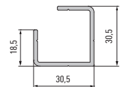
928 128 Corner profile
