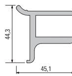
902 181 Support profile for 16 mm base
