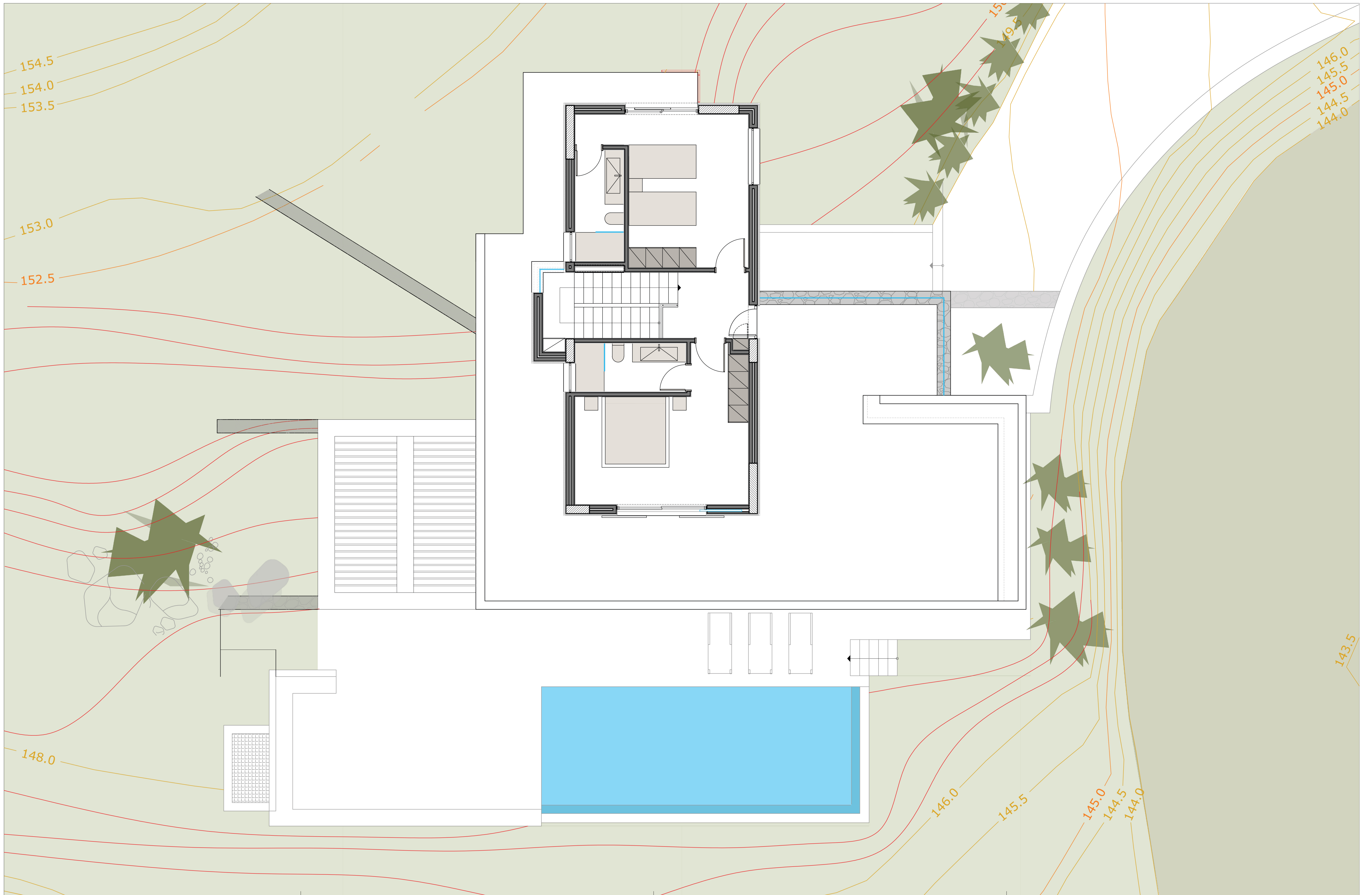
UPPER FLOOR PLAN
