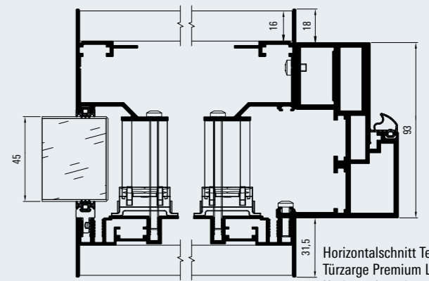
Horizontalschnitt Technikpaneel Türzarge Premium S Horizontal section detail for technical panel for premium door frame trim S
