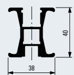
Griffprofil 40 C Handle profile 40 C 100008319
