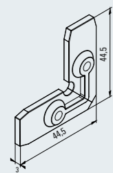
Eckverbinder Türprofil Premium L-XL Corner cleat, premium door profile L-XL 100011927
