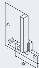
Adapter Träger Adapter for load-bearing profile 100022338
