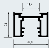
Griffprofil 16 Handle profile 16 100008660
